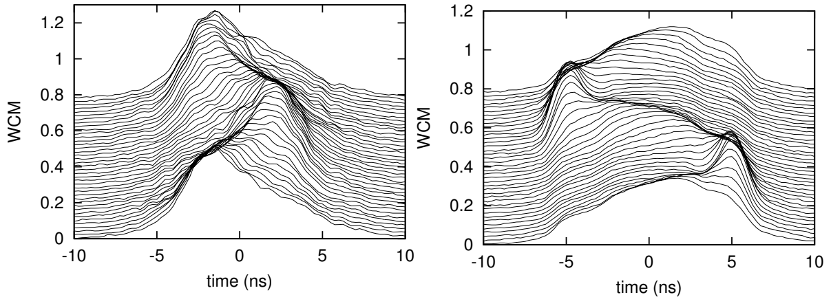
Figure 4.2: Wall current monitor data for a freshly injected (left) bunch of protons with \gamma = 35.9 at RHIC and the same bunch 17 min later, still at injection energy (right).
