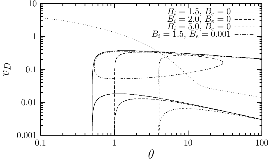
Figure 2.10: Negative energy areas of the \theta , v_D plane for ion holes with different values of B_e and B_i satisfying B_i + \frac{3}{2}B_e > 1 . The vertical lines where the curves for B_e = 0 abruptly cease are given by \theta = \theta_0 . Note the shrunk area of \Delta w < 0 in case of B_e = 0.001 . The dotted line represents the linear stability limit.
