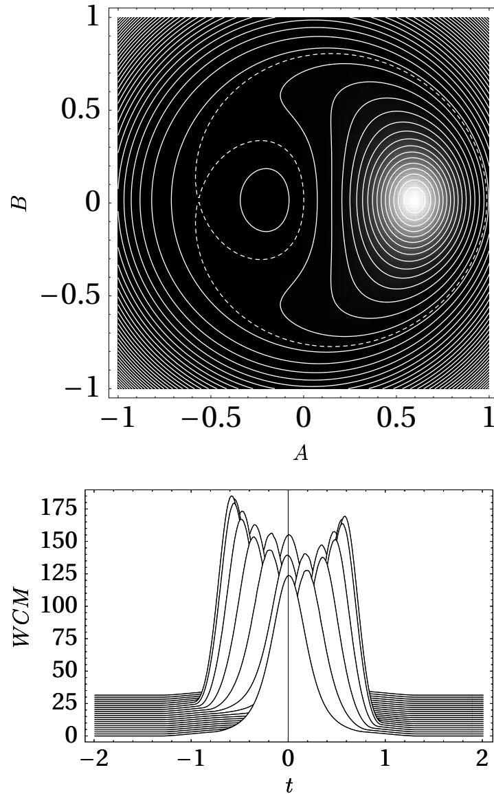
Figure 4.7: (a) Phase space density (gray scale) and contours of constant energy K(A, B) (particle trajectories). (b) Line density (simulated WCM data). The solution was obtained with \alpha = 0.3 , \tilde{r} = 0.025 , C_1 = 0.1 , C_3 = 0.005 , \ell = 0.01 , C_0 = 21975 and \psi = 0.014 . This solution consists in a large soliton with a little background, i.e., almost all particles are trapped in the soliton.
