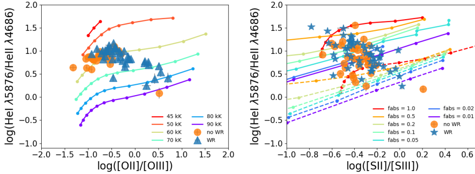
FIGURE 2. Examples of two softness diagrams for the sample of He II-emitters presented in Pérez-Montero et al., 2020. At left [[\text{O II}]]/[[\text{O III}]] vs He I/He II/ with models at 12+\log(\text{O}/\text{H}) and different values for T_{\text{eff}} and, at right, using [[\text{S II}]]/[[\text{S III}]] and BPASS models assuming different values for f_{\text{abs}} . In all sequences values in the lower left part correspond to higher values for \log U .
